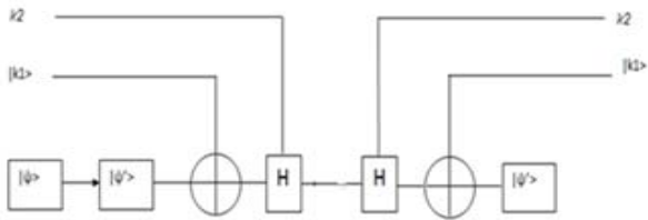
Fig. 3: Qubit of encryption and decryption
