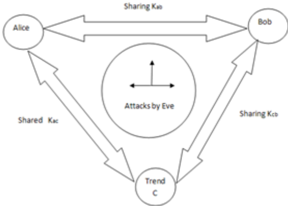
Fig. 2: Distribution of the quantum keys for blind signature.
